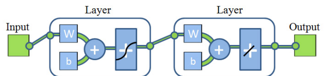
Fig. 2 Neural Network Model Structure of Grass Carp Hemorrhage Prediction
