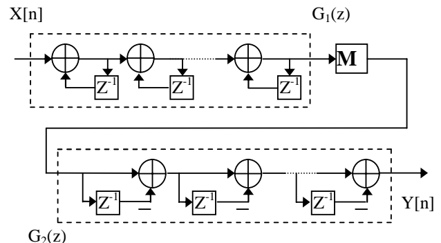
Fig. 1 Decimation filter
