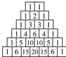
Fig. 2 The Pascal's triangle
