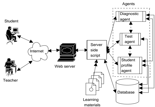
Fig. 6. System architecture
