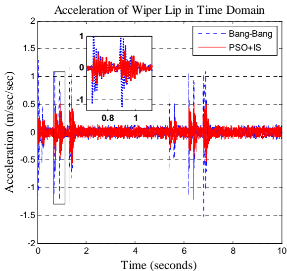
Fig. 16 end point acceleration in y- direction
