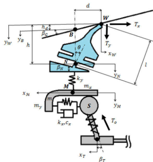
Fig. 1 Spring-mass model wiper blade system [12]
