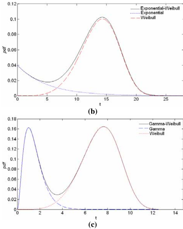
Fig 1. The graphs of the mixture models of two different distributions for simulation parameters
