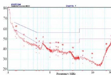
Fig.7 Conducted Emissions with Common Mode Filter
