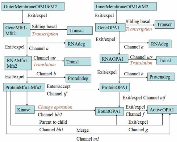
Fig. 1 Diagrammatic representation of the proposed model, where M1 and M2 are two independent mitochondria of the same cell
