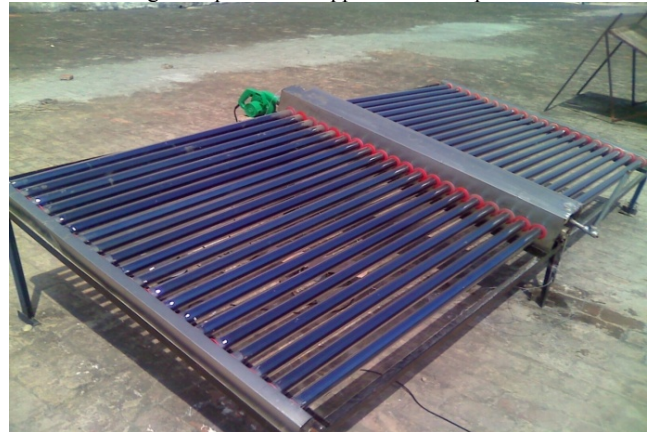
Fig.3 Experimental apparatus with down flow
