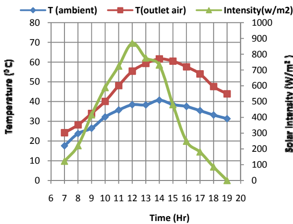
Fig.13 Variation of air collector inlet air, out let air and radiation intensity during day 162.86 m³/hr air flow rate
