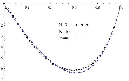
Fig. 1. Exact and approximate solutions for Example 1, ( N = 3, 10 ).
