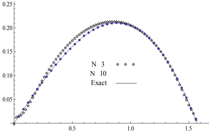
Fig. 2. Exact And Approximate Solutions For Example 2,( y_1 ).
