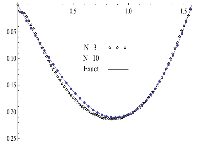
Fig. 3. Exact and approximate solutions for Example 2,( y_2 ).
