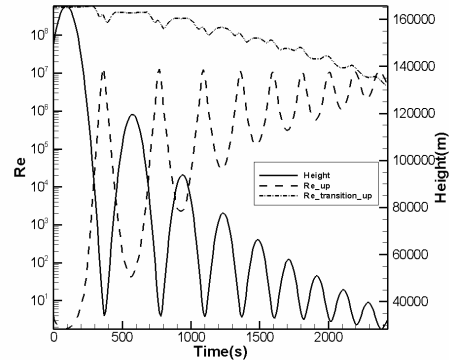
Fig. 4 Transition analysis on the upper surface
