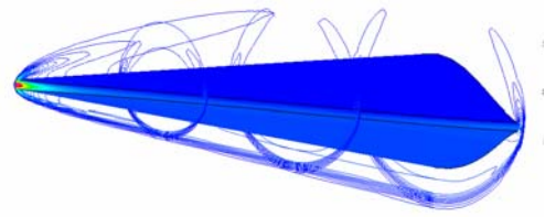
Fig. 8 Pressure contours around the HGCV
