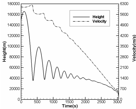
Fig. 2 Height and velocity varied with time
