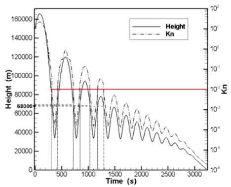
Fig. 3 Knudsen number and height varied with time
