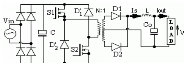
Fig. 1 Main system of arc welding machine
