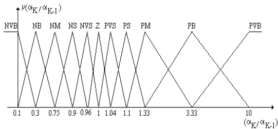
Fig. 6 Membership functions for Phase-shift angle ( \alpha_k/\alpha_{k-1} )
