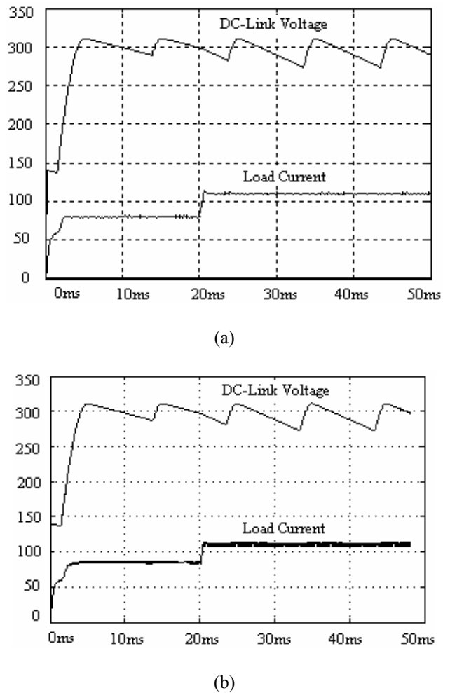
Fig. 10 DC-link voltage and load current for filter inductance of 75 \mu H a) by FLC b) by Sliding
