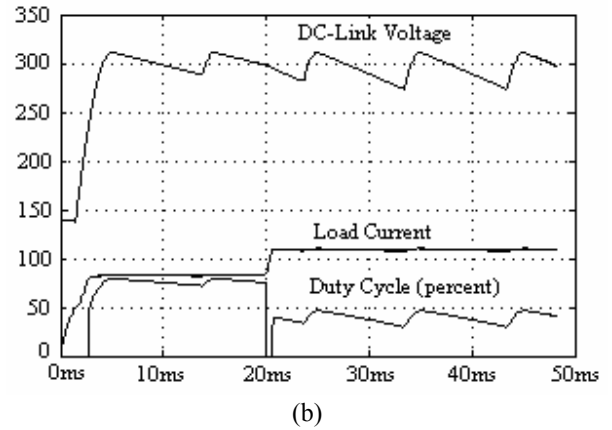
Fig. 9 DC-link voltage, phase-shift angle and load current a) using FLC b) using sliding mode control
