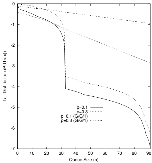
Fig. 3 The effect of correlations on performance
