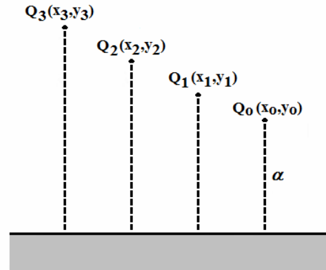
Fig. 2 Definition diagram of multiple sea outfalls
