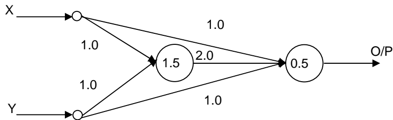
Fig. 2 Realization of XOR function using two neurons.
