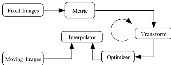
Fig.2 The basic components of the registration framework are two input images, a transform, a metric, an interpolator and an optimizer
