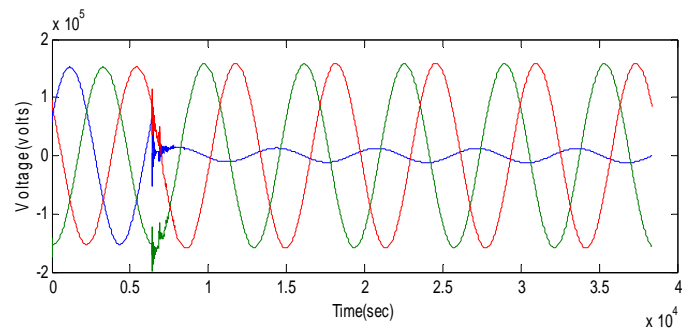
Fig. 3 Three phase voltage at terminal X
