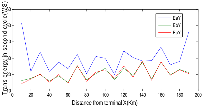
Fig. 11 Transient energy at Y in the second cycle (when single LG fault occurs)
