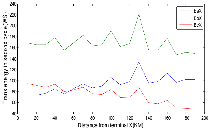
Fig. 18 Transient energy at X in the second cycle (when LLLG fault occurs)
