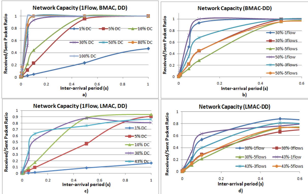
Figure 2: Successful Transmission Measurements Excluding Routing Protocol Overhead
