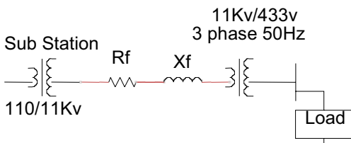
Fig.4 Single Line Diagram of Distribution System
