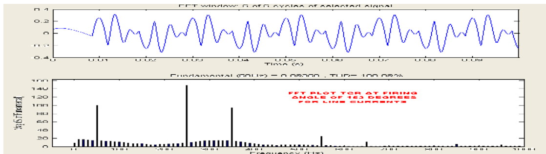
Fig.22 Harmonic spectrum for line current at \alpha = 153^0
