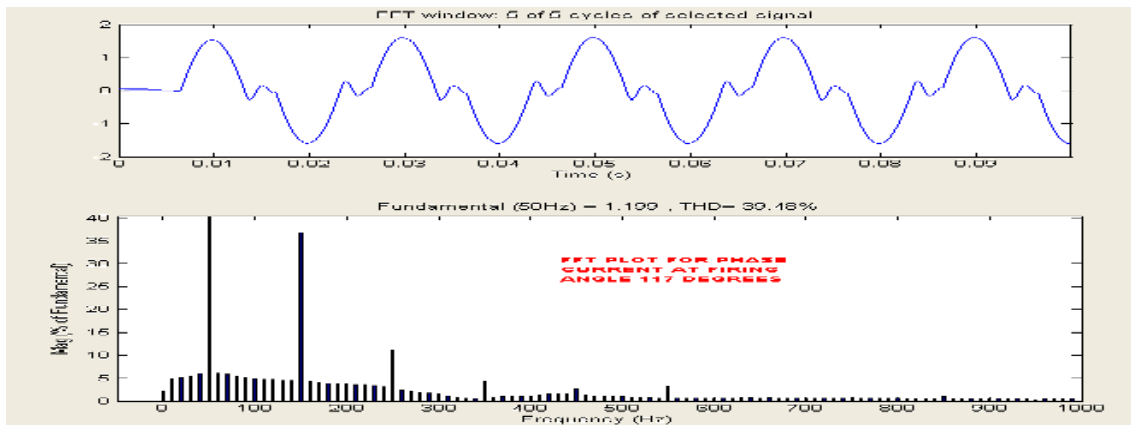
Fig. 18 Harmonic spectrum for phase current at \alpha = 117^\circ
