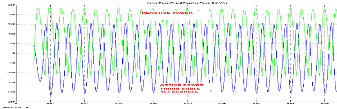
Fig20 Active reactive power at \alpha = 153^0
