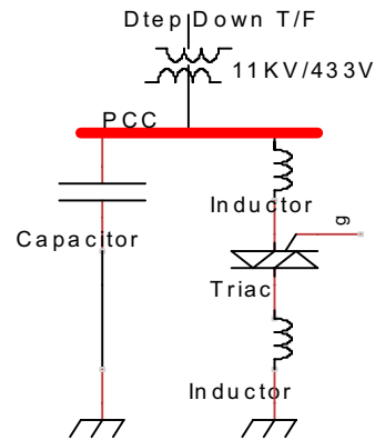
Fig. 6 FC-TCR Scheme
