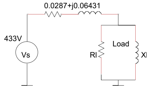
Fig.5 Parametric Diagram on L.V. Side
