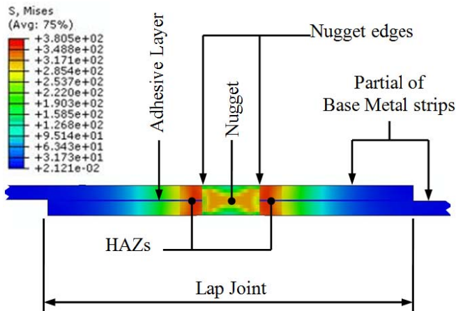
Fig. 9 Contour residual stresses for FE weld-bonded model
