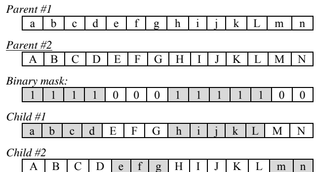
Fig. 3 Applying a binary mask on parent #1 and parent #2 produces child #1 and child #2
