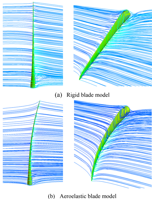
Fig. 8 Comparison of instantaneous pressure contours with stream lines of the 5 MW class wind-turbine blade.
