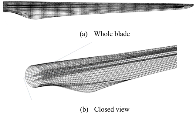
Fig. 4 Finite element structure of blade
