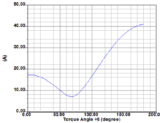
Fig. 14 Line current versus torque angle
