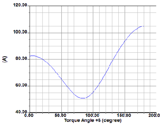
Fig. 8 Line current versus torque angle
