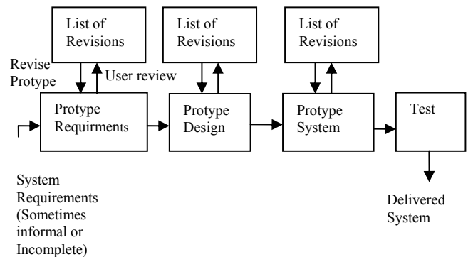
Fig. 4 Iterative Method Outline
