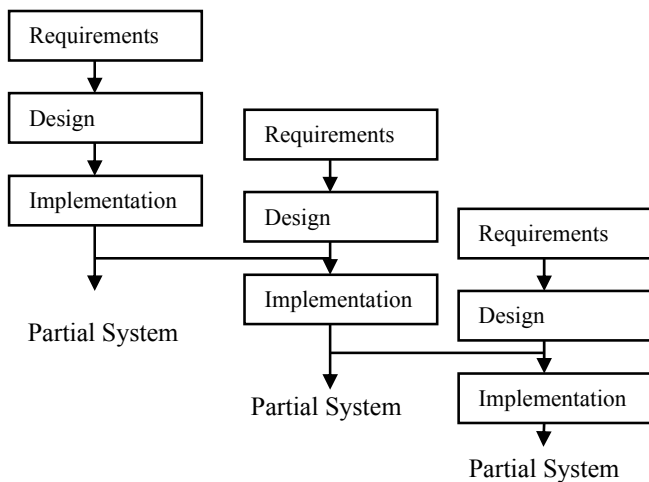
Fig. 3 The Iterative Model
