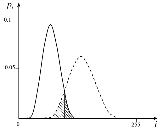
Fig. 1 Classification error for mixture of two Gaussians
